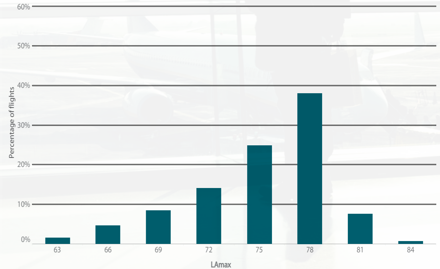
Figure 33: L_{A,MAX} levels distribution for NMT 5, January - June 2018. Updated in September 2020 (see executive summary).
