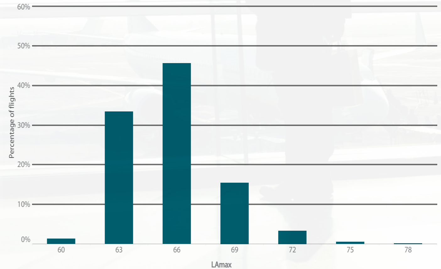
Figure 26: L_{A,MAX} levels distribution for NMT 4, January - June 2018. Updated in September 2020 (see executive summary).
