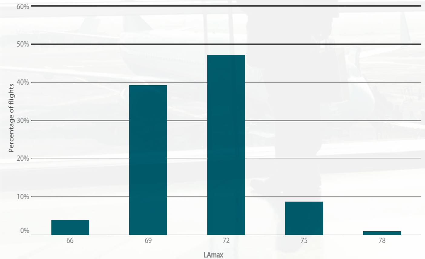
Figure 47: L_{A,MAX} levels distribution for NMT 20, January - June 2018. Updated in September 2020 (see executive summary).
