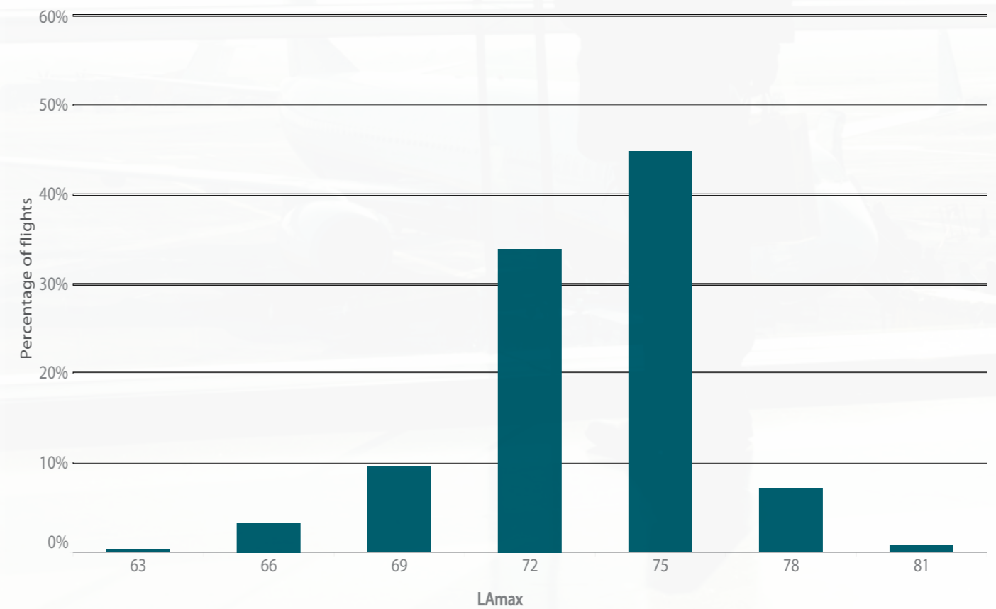
Figure 19: L_{A,MAX} levels distribution for NMT 2, January - June 2018. Updated in September 2020 (see executive summary).
