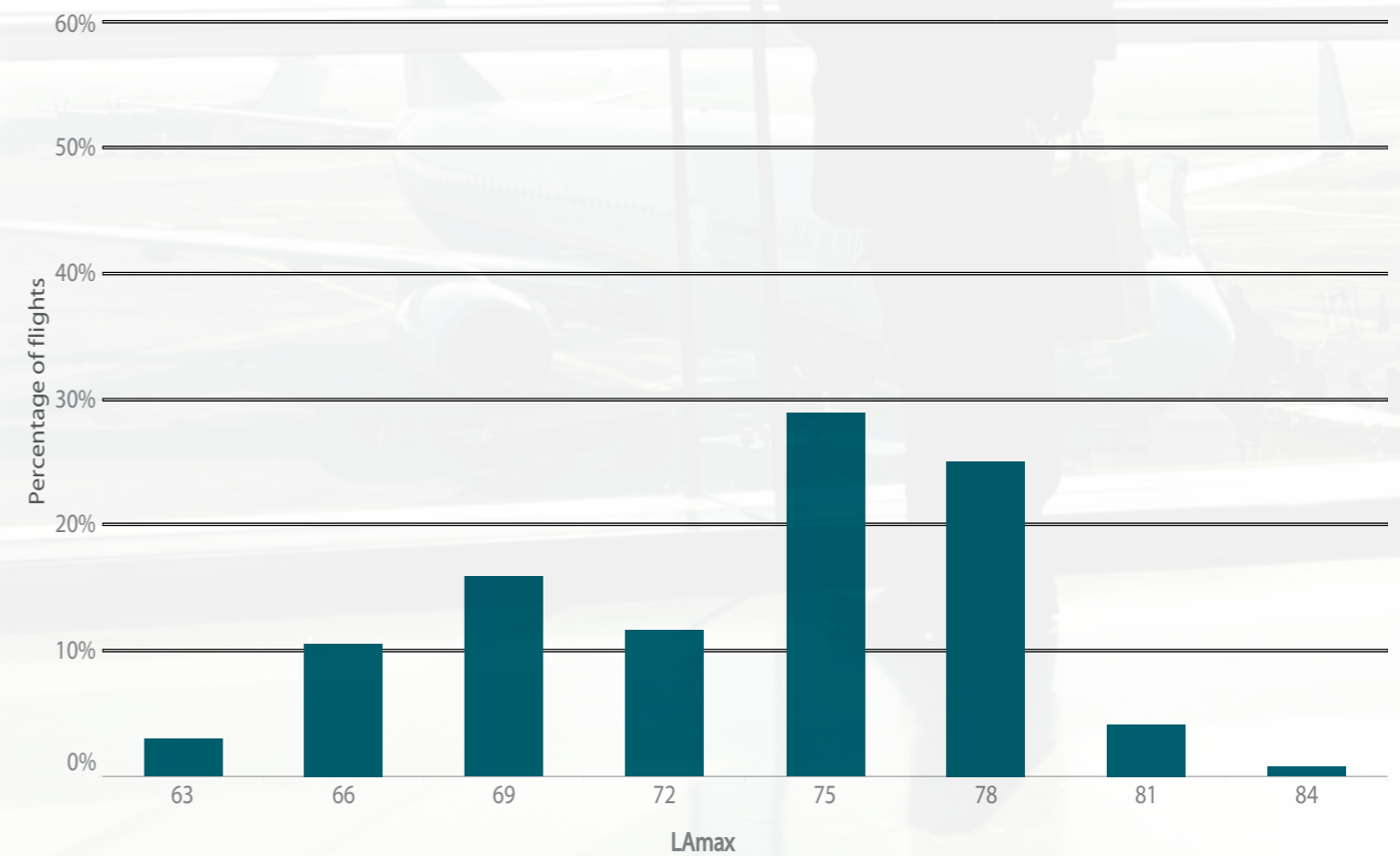
Figure 40: L_{A,MAX} levels distribution for NMT 6, January - June 2018. Updated in September 2020 (see executive summary).
